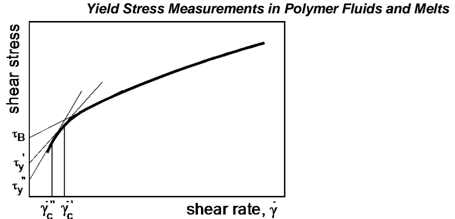
Figure 4: Extrapolation of constant shear stress values to zero shear rate in order to calculate yield stress. The value of the yield stress will depend on the shear rate from which the extrapolation is made.
