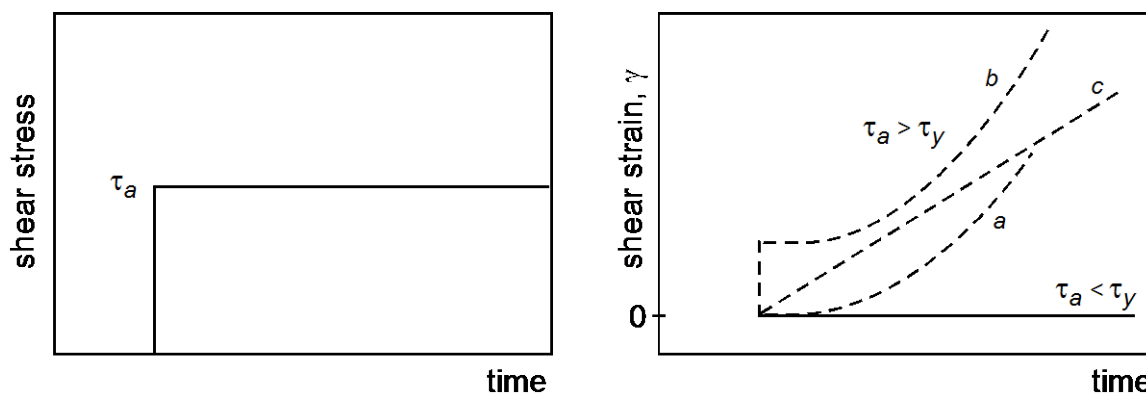
Figure 1: Behavior of material under a step change in stress. Dashed lines in resultant shear strain are for cases where the applied stress is greater than the yield stress.
